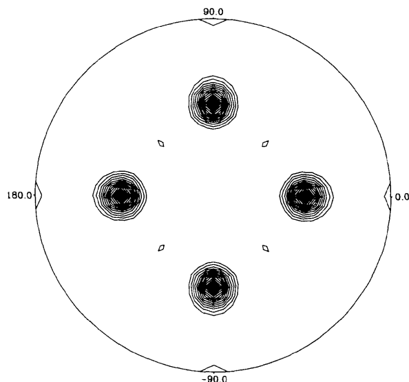
Fig. 2. A stereographic plot of the \kappa = 120^\circ section of the self-rotation function for the vanadium-dependent bromoperoxidase native data ( 40\text{--}4 \text{ \AA} ). The positions of the four non-crystallographic threefold axes can be clearly seen. Plot contoured at 5\sigma levels above 10\sigma .
